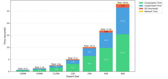
Figure 2: Time Components in Traditional Disk-Based Expert Loading
