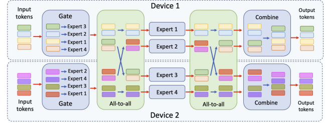
Figure 1: MoE architecture[22]
